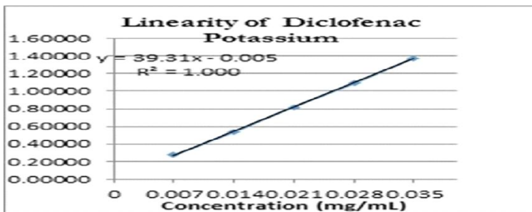
Fig. 1. Standard curve of Diclofenac Potassium
