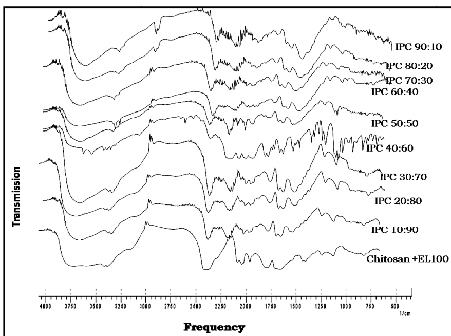
Fig. 5. FTIR spectra of all the IPEC solution, Chitosan+EL100
