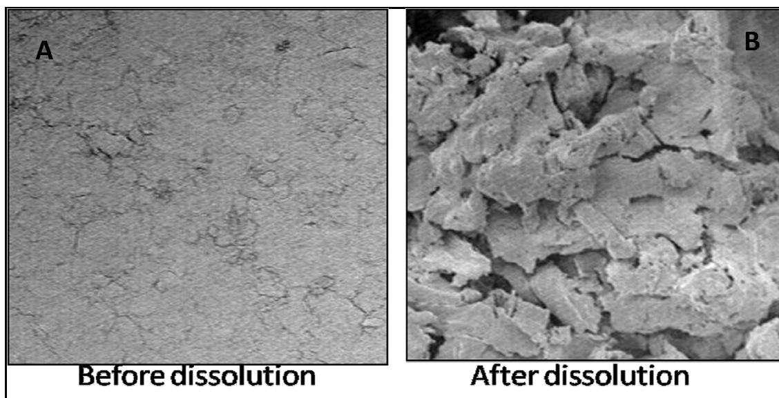
Fig. 8. SEM photographs of C7 tablets showing surface morphology (A) before and (B) after dissolution study
