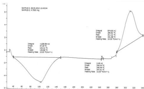
DSC thermogram of Chitosan
