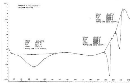
DSC thermogram of IPEC 40:60 + Diclofenac Sodium
