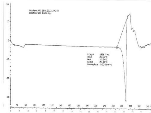
DSC thermogram of Diclofenac Sodium
