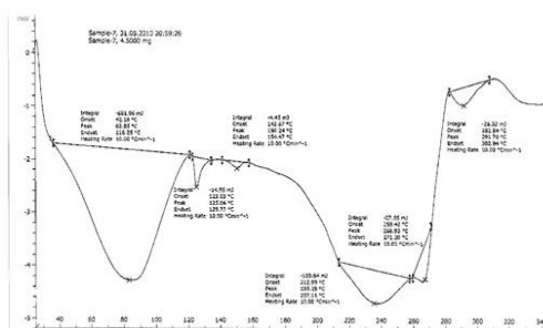
DSC thermogram of Chitosan + Eudragit L100 + Diclofenac Sodium
