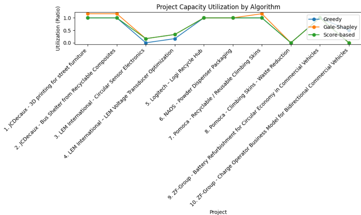
Fig. 1. Project capacity utilization by algorithm
