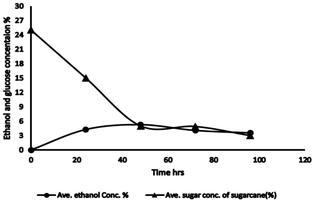
Fig. 3. Ethanol and Glucose concentration from sugarcane juice
