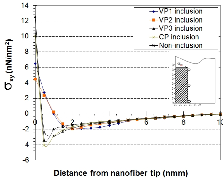
Fig. 8. Shear stress \sigma_{xy} along the long side of the nanofiber due to vertical inclusion
