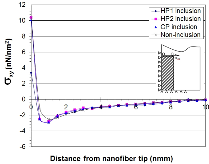
Fig. 9. Shear stress \sigma_{xy} along the short side of the nanofiber due to horizontal inclusion
