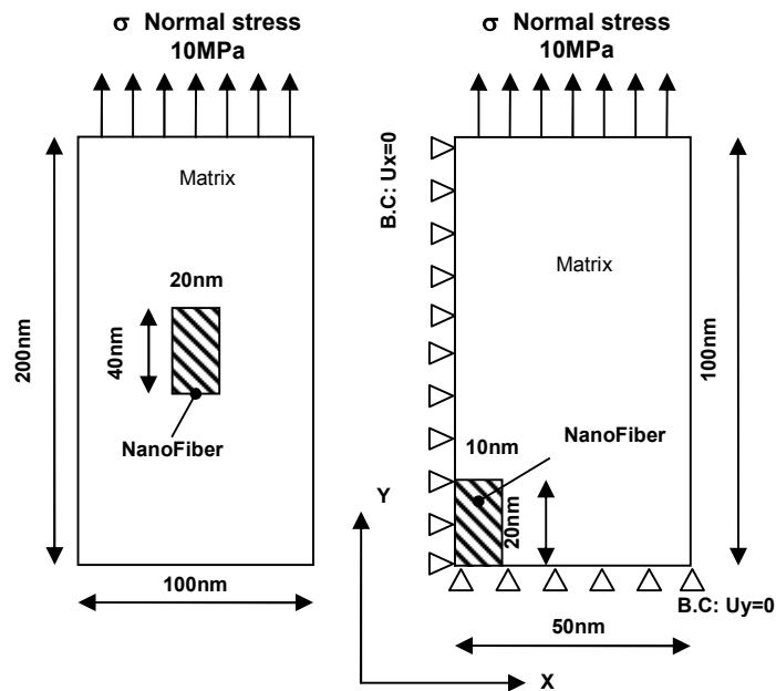
Fig. 1. Dimensions and boundary condition of the RVE used for FEA
