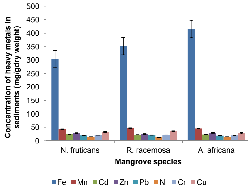
Fig. 2. Concentration heavy metals in the mangrove sediments
