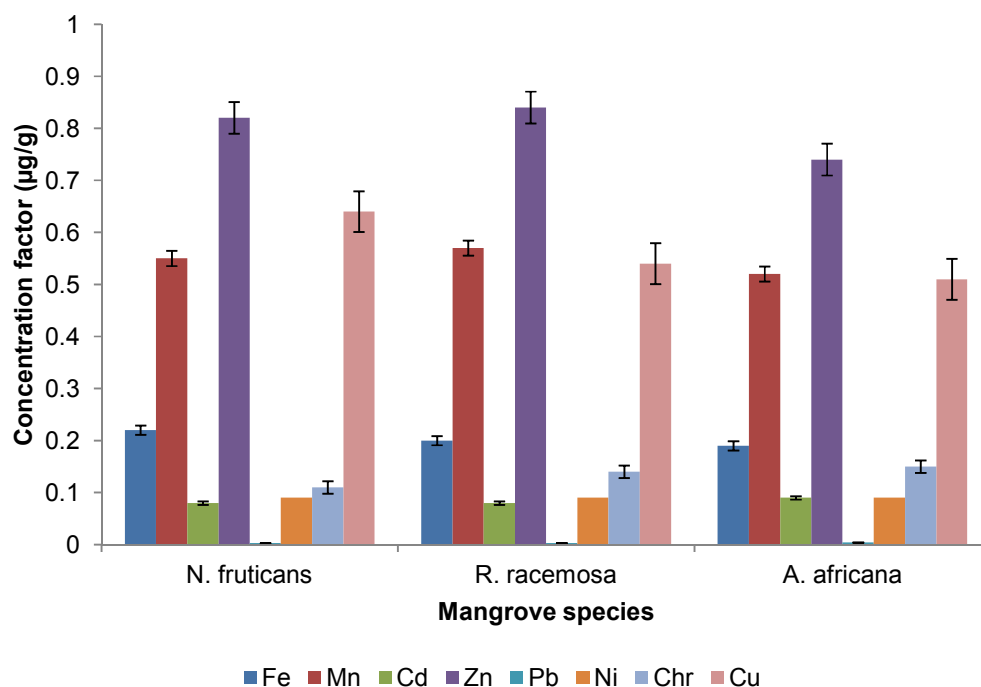
Fig. 3. Concentration factor for heavy metals in the mangrove sediment and plant tissues
