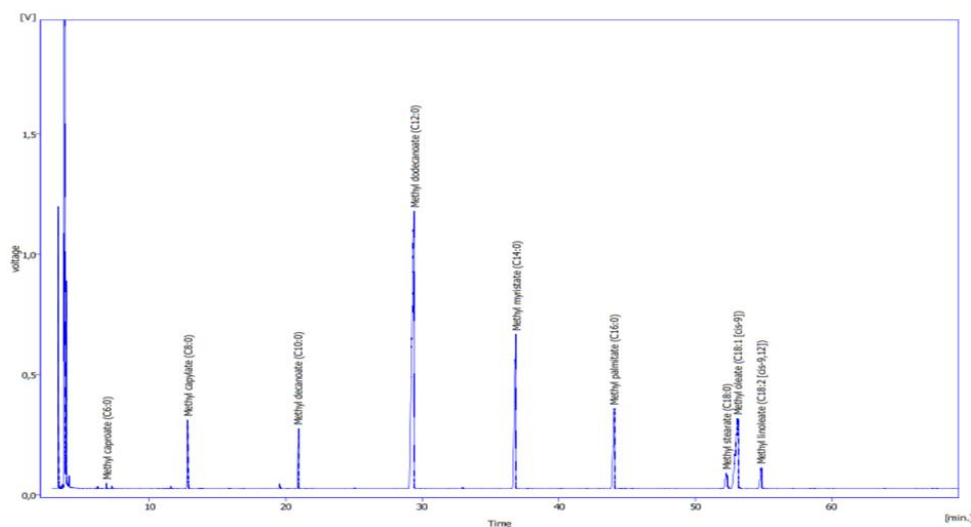
Fig. 2. Chromatogram for methyl esters of fatty acids (FAME) of oil D
