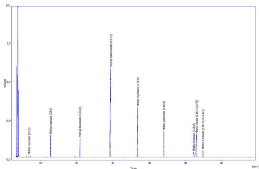
Fig. 3. Chromatogram for methyl esters of fatty acids (FAME) of oil D
