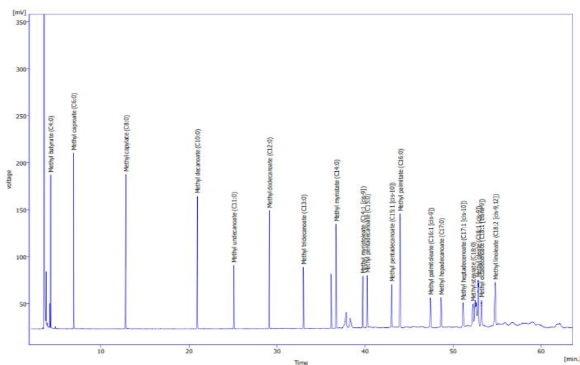
Fig. 1. Chromatogram for standards methyl esters of fatty acids (FAME) mix
