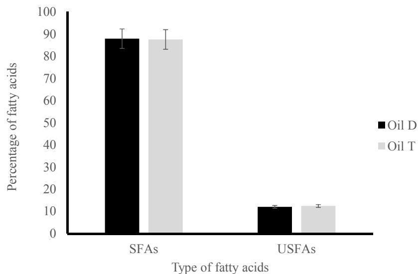
Fig. 4. Total saturated and unsaturated fatty acids of the oils analyzed
