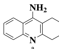
Fig. 4. Tacrine
