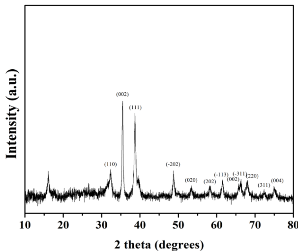
Fig. 4. Powder XRD pattern of CuO NPs using Coix lacryma jobi leaves extract
