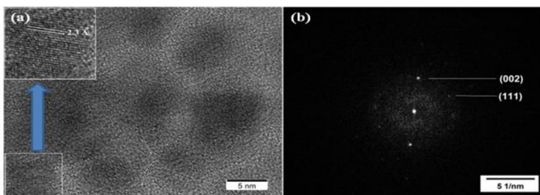
Fig. 5. (a) HRTEM image of CuO NPs with inset showing d spacing (b) SAED pattern
