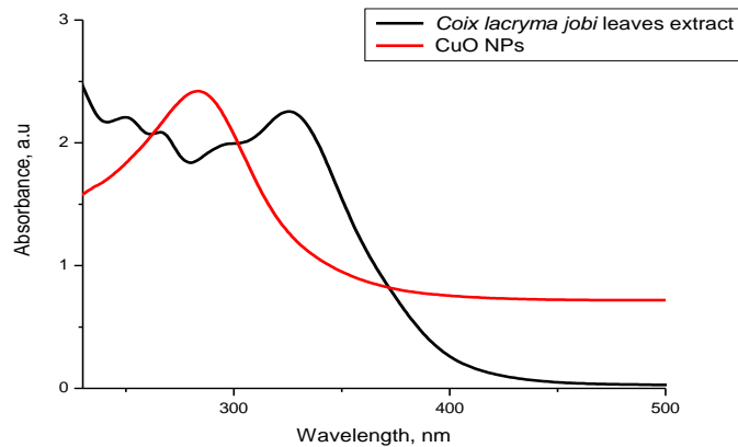
Fig. 3. UV-Visible spectra showing absorption of 10^{-3} M aqueous solution of green CuO NPs (red curve) and Coix lacryma jobi leaves extract (black curve)
