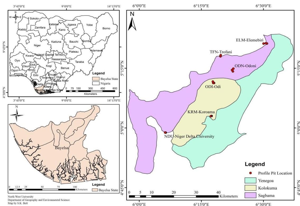
Fig. 1. Map of Bayelsa State showing study locations and rivers linked to the Atlantic Ocean (source: Dickson,[8])
