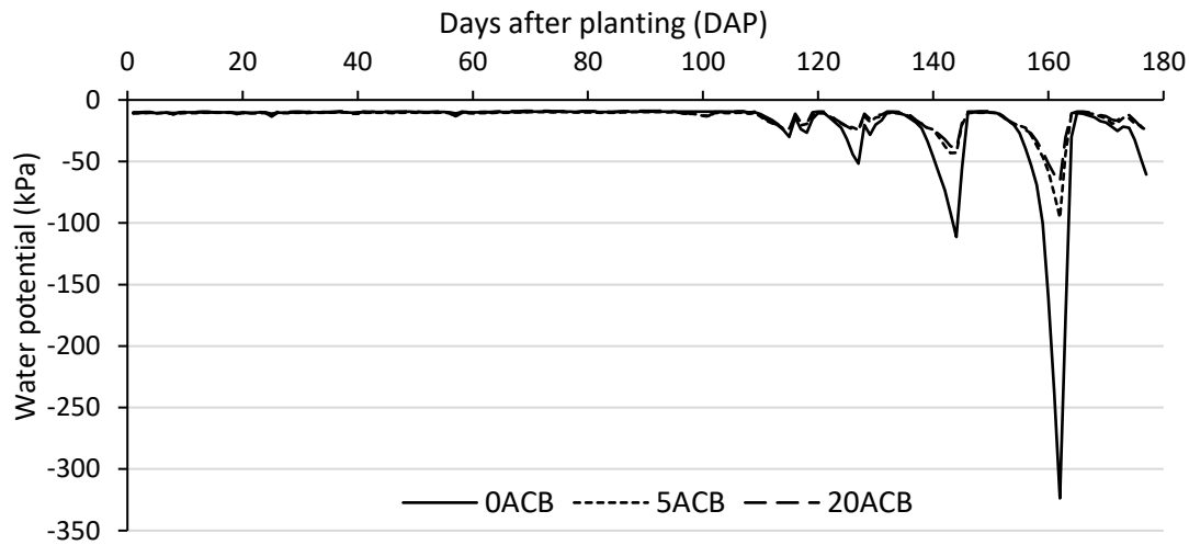
Fig. 6. Effects of biochar application on soil water potential at 10 cm depth
