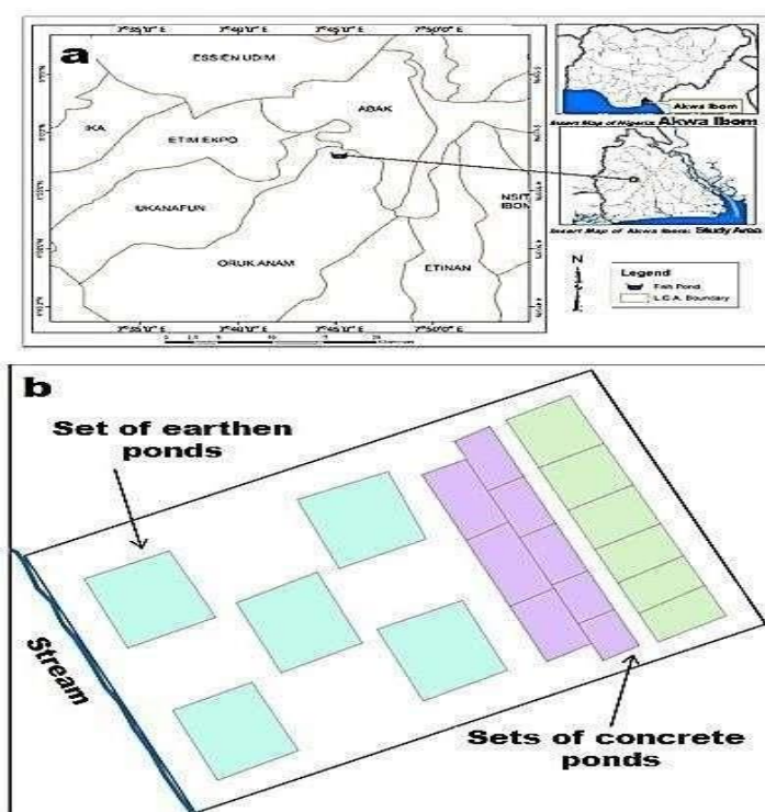
Fig. 1. A cross section of map of Nigeria showing Akwa Ibom with an inset showing the location (a) and layout (b) of the University Fish Farm Complex
